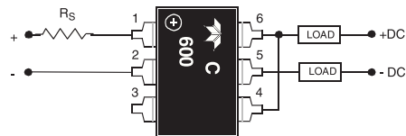
B) DC CONFIGURATION (SEE NOTE 4)
