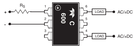
A) BI-DIRECTIONAL/AC CONFIGURATION (SEE NOTE 4)
