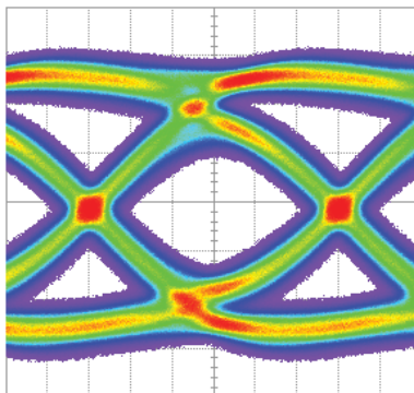
GRF121A/GRF121AR @ 40Gbps
