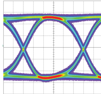
Reference @ 16Gbps
