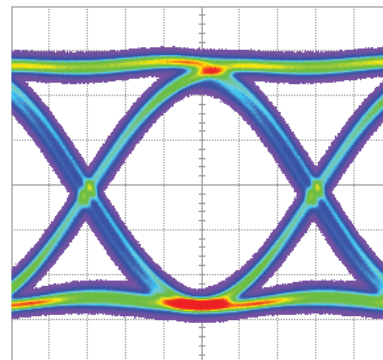
Reference @ 40Gbps
