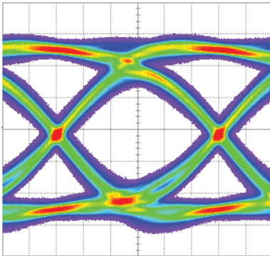
GRF121A/GRF121AR @ 28Gbps
