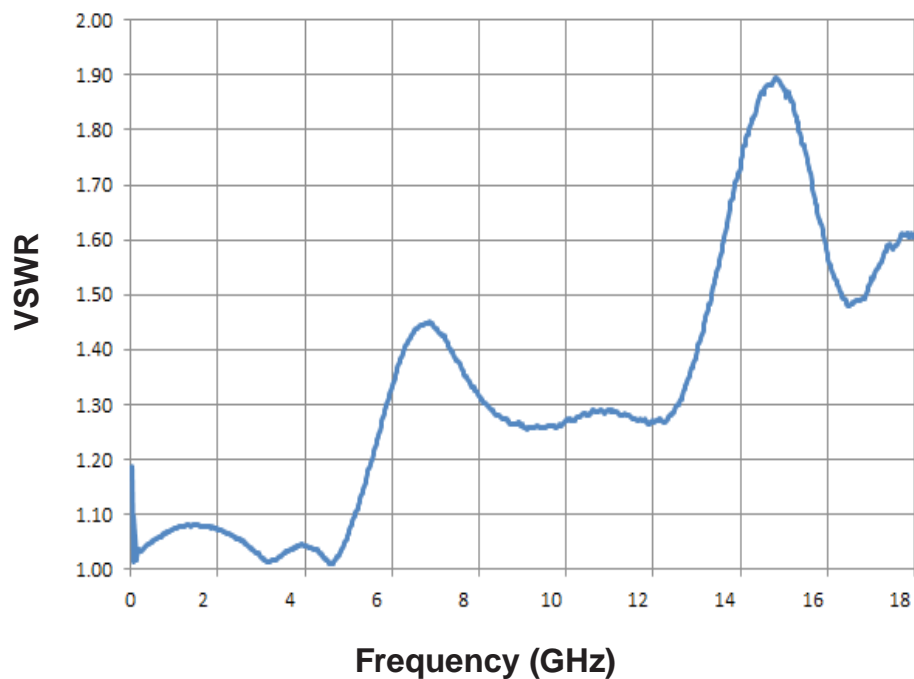
VSWR (RF Note 3)
