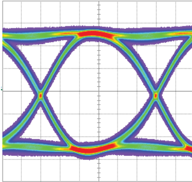
GRF121A/GRF121AR @ 16Gbps
