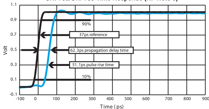
GRF700/GRF703 Time Response (RF Note 6)
