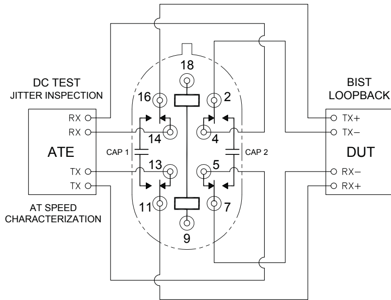
(Contacts shown in De-Energized position)
